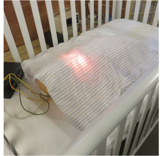
Supplementary Figure 2 – Test setup for pacifier and receiving blanket over the face.
