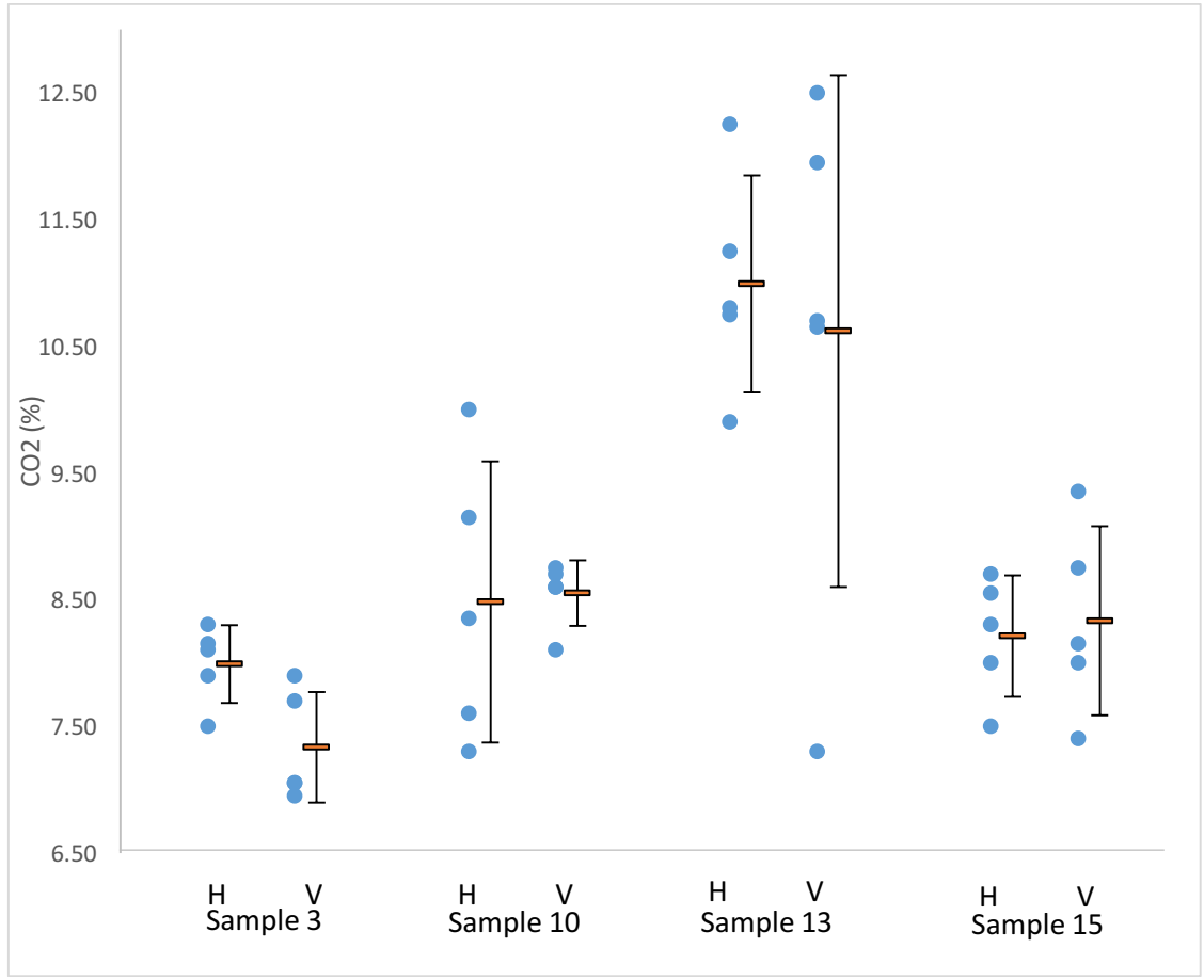
Supplementary Figure 1 – CO 2 RB in horizontal (H) and vertical (V) crib side positions. Error bars represent mean and standard deviation.
