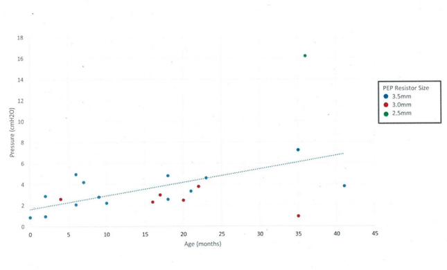
Figure 1 Scatterplot age versus pressure.
